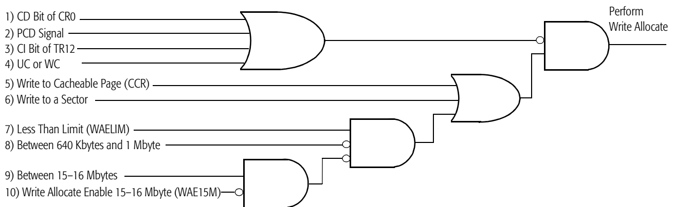
Figure 77. Write Allocate Logic Mechanisms and Conditions
