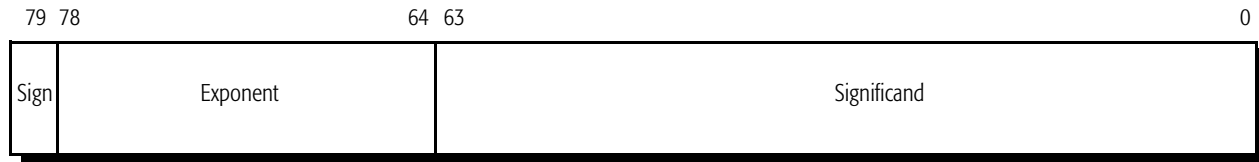
Figure 11. Floating-Point Register
