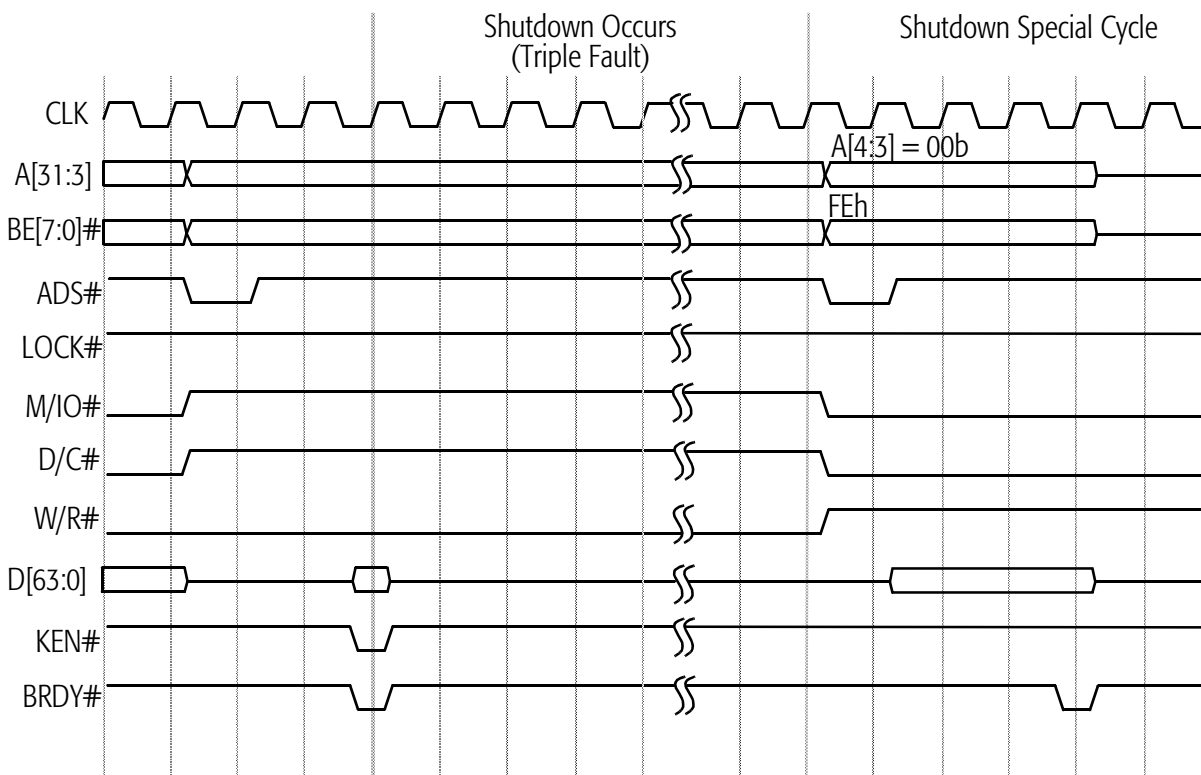
Figure 70. Shutdown Cycle
